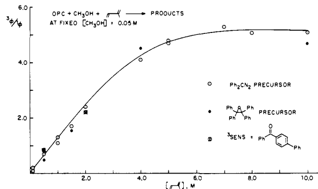
Figure 1. The ratio of cyclopropanes to ether ( 3 φ/ 1 φ) formed by reaction of DPC in acetonitrile solvent, at fixed (0.05 M) concentration of methanol and variable concentrations of isoprene.
